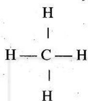
Methane
